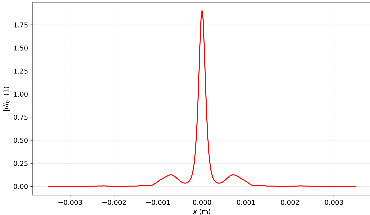
Intensity profile I(x, y = 0, z = 1.672)/I_0 , P_{in}=8.0P_{cr} , artificial time
